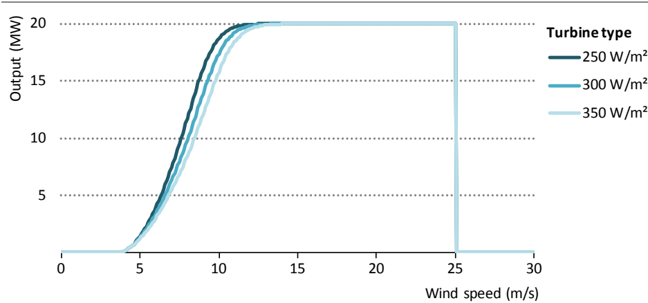
Figure B.2 ▶ Illustrative power curves for 20 MW wind turbines
