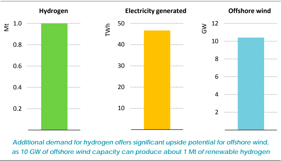
Figure 29 ▶ Offshore wind capacity needed to produce 1 Mt of hydrogen
