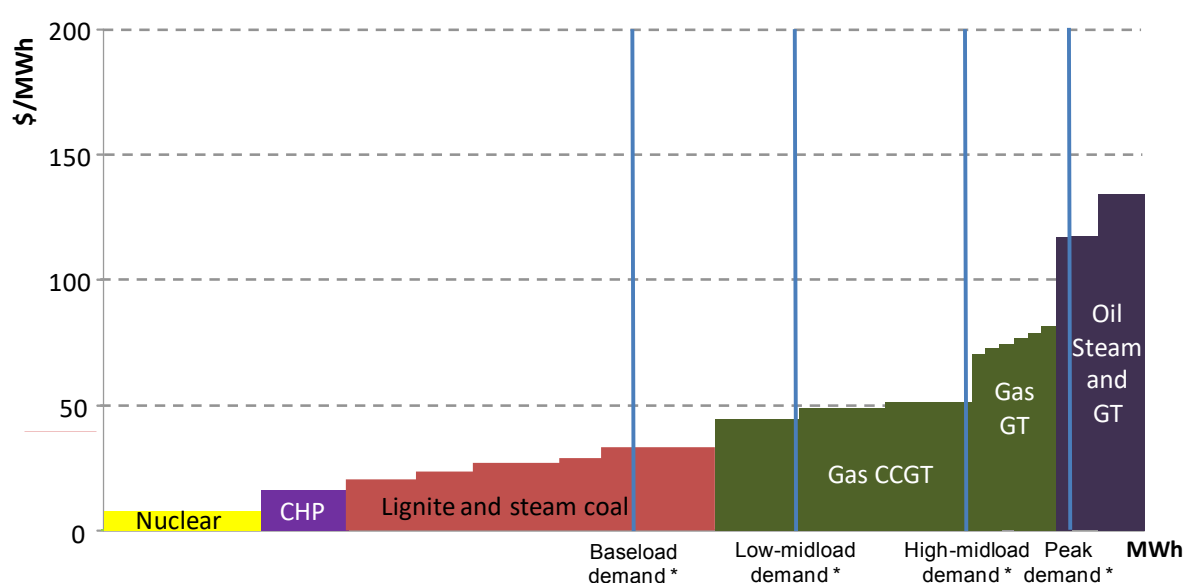
Figure 4.3 ▶ Example merit order and its intersection with demand in the power generation module
