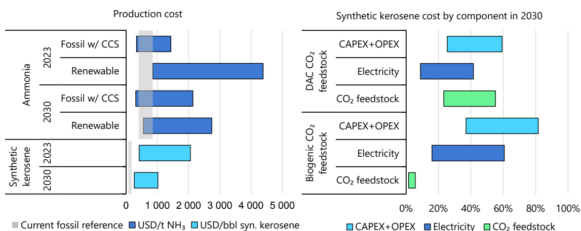
Figure 3.19 Levelised costs of ammonia and synthetic kerosene for electricity-based pathways in 2023 and in the Net Zero Emissions by 2050 Scenario in 2030
