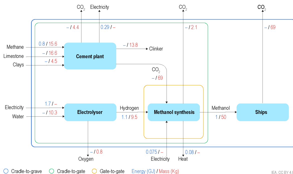
Figure 7.10 Alternative boundary definitions used to account for GHG emissions from methanol using CO 2 sourced from a cement plant
