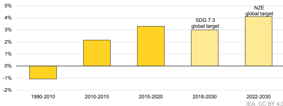
Figure 4.4 Annual rate of energy intensity improvements in Senegal (1990-2020) and global targets until 2030
