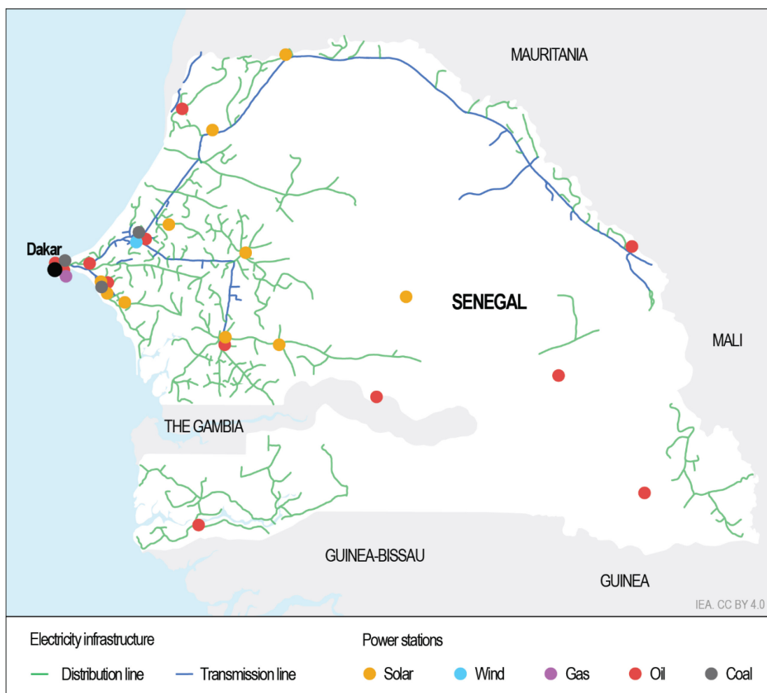
Figure 6.5 Electricity infrastructure and power plants in Senegal
