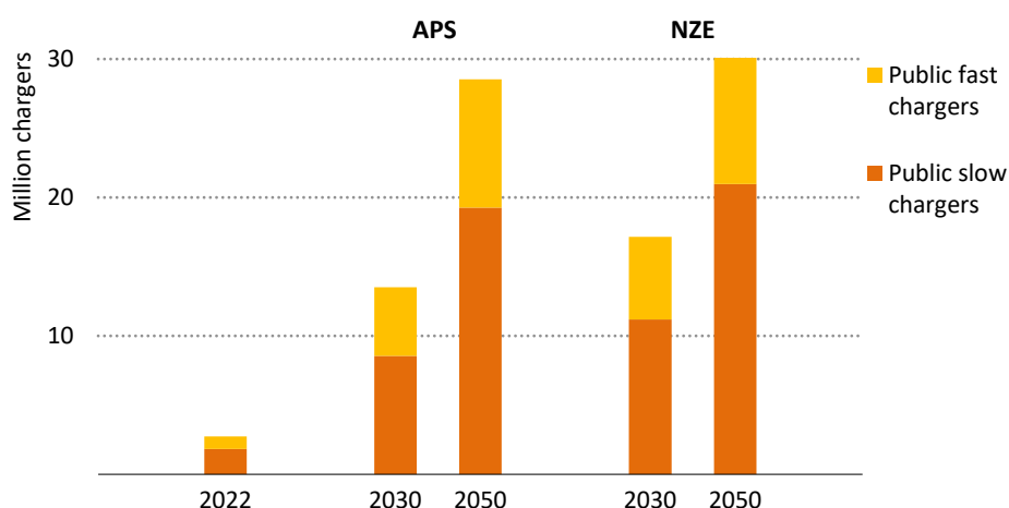
Figure 2.34 ▶ Projections for electric light-duty vehicle chargers in the APS and NZE Scenario, 2022-2050
