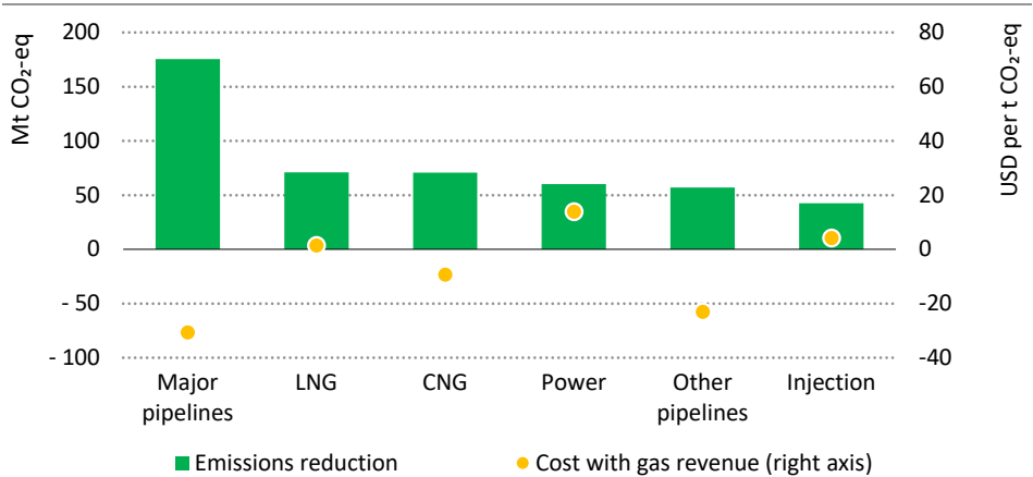
Figure 2.10 ▶ Emission reduction potential and average cost of flaring reduction measures in the NZE Scenario, 2022
