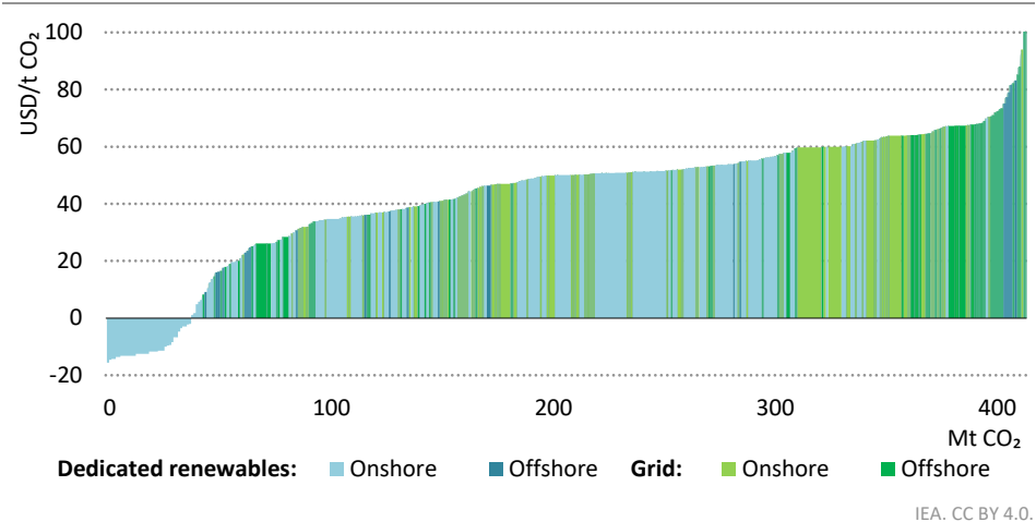
Figure 2.11 ▶ Cost of electrifying oil and gas production sites
