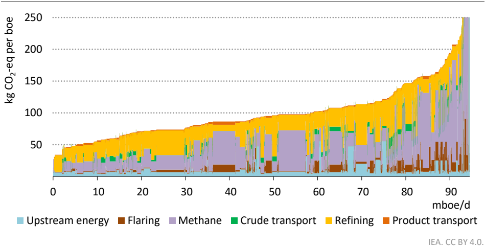
Figure 2.2 ▶ Spectrum of scope 1 and 2 emissions for oil, 2022
