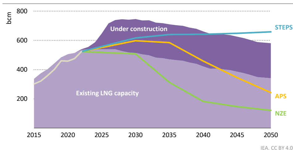
Figure 1.18 ▶ Existing and under-construction LNG liquefaction capacity and LNG trade by scenario
