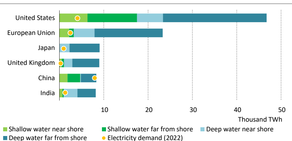
Figure 2.29 ▶ Offshore wind potential and 2022 electricity demand in selected regions and countries
